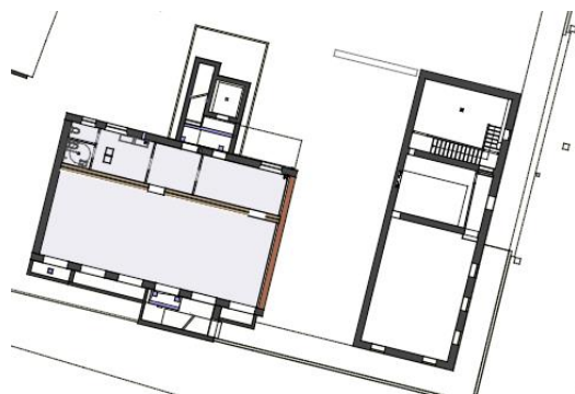
PIANO SEMINTERRATO
