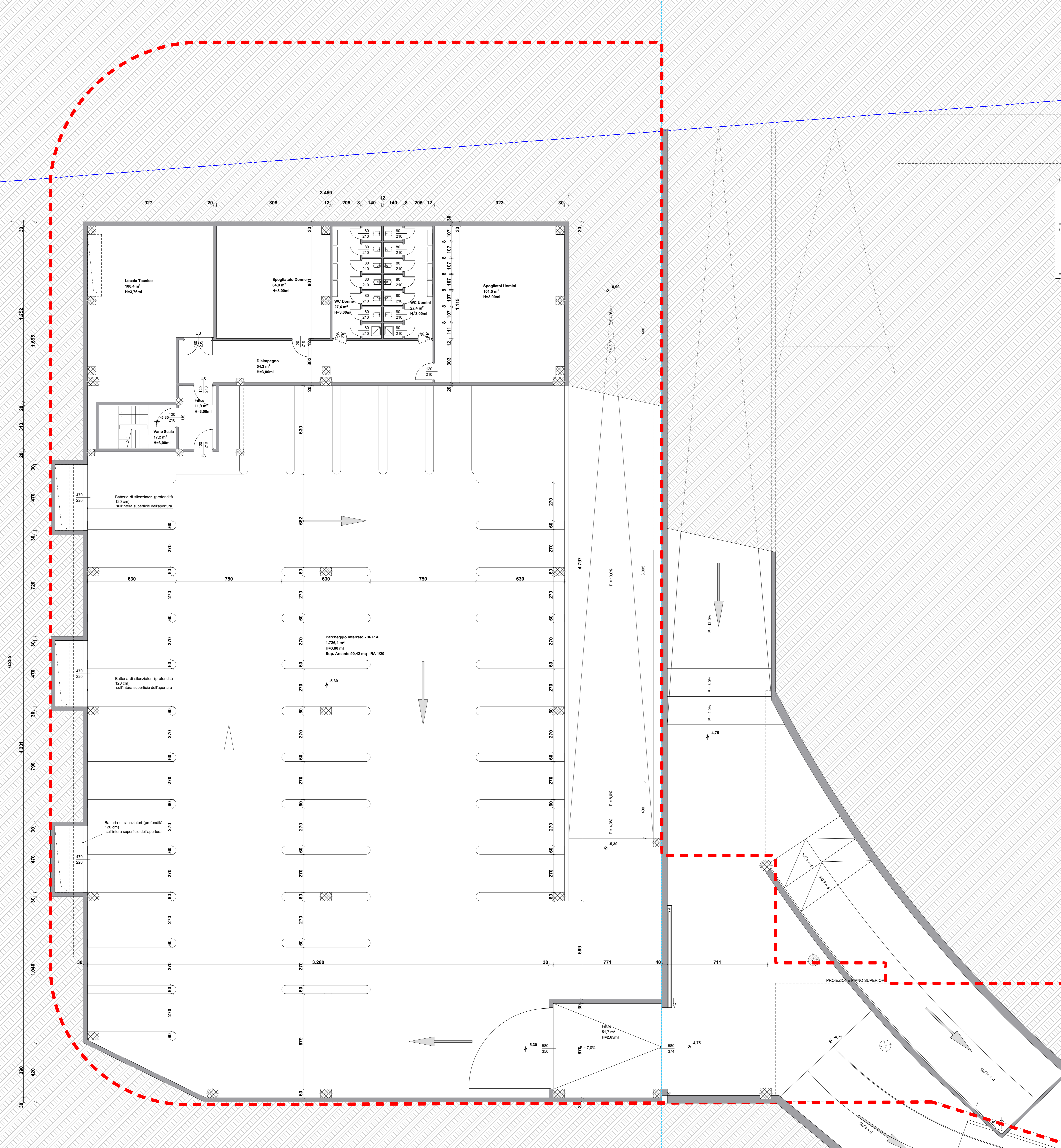
Piano Interrato
